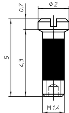
Screw – 28.3163000.N92
